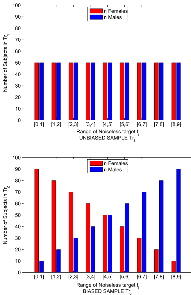
Fig. A.12. No of subjects by gender over unit intervals of f_i in the unbiased training sample T_1 are shown in (a). The corresponding barchart for the biased training sample T_2 is shown in (b).
