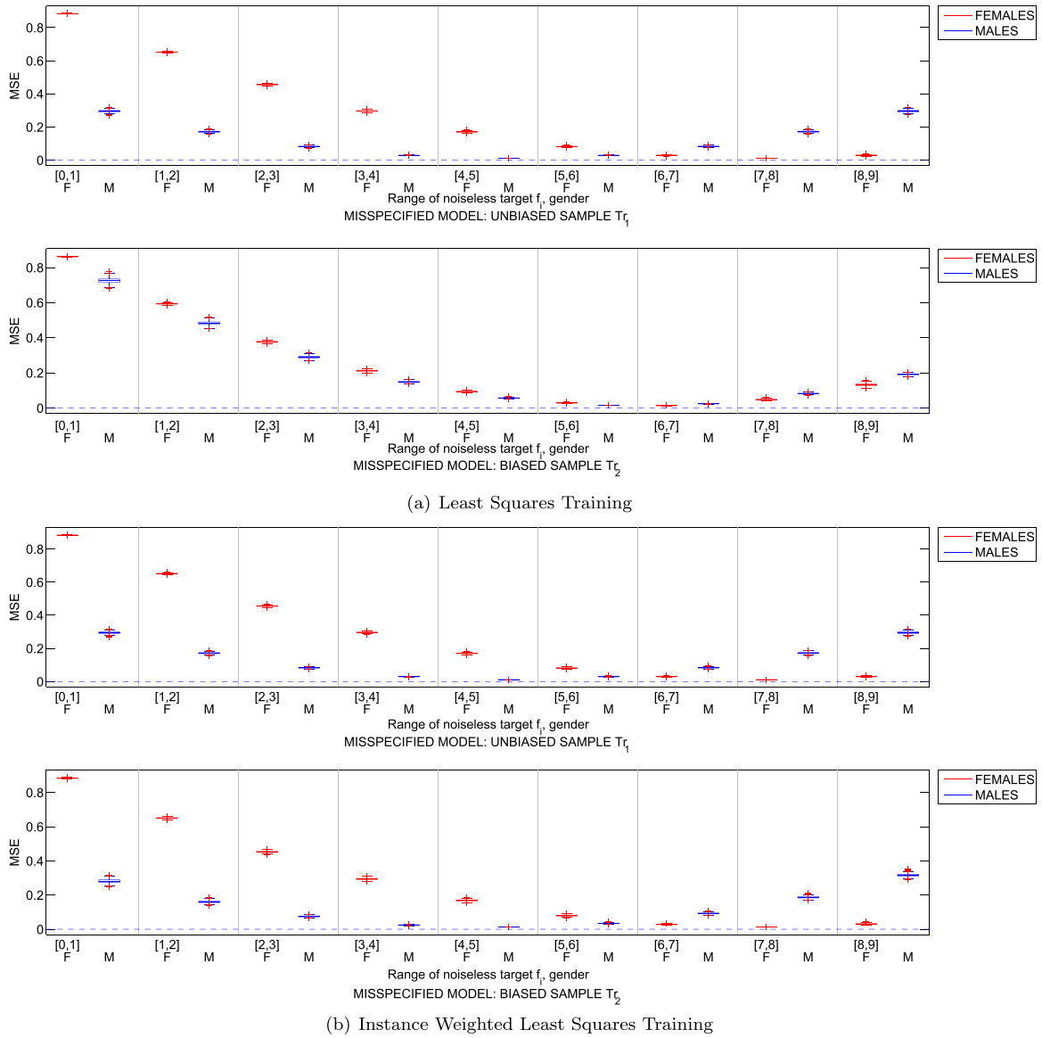
Fig. A.14. Results using least squares training are shown in (a), while (b) shows results using Instance Weighted least squares. In both figures, the top row shows the MSE as the value of the noiseless target f_i changes, for each gender, when training using the unbiased sample T_1 and a misspecified model. The bottom row in each figure shows the corresponding boxplot when using biased sample T_2 .
